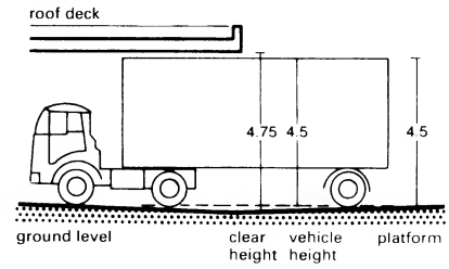
12 Dimensions for sheltered loading bays
